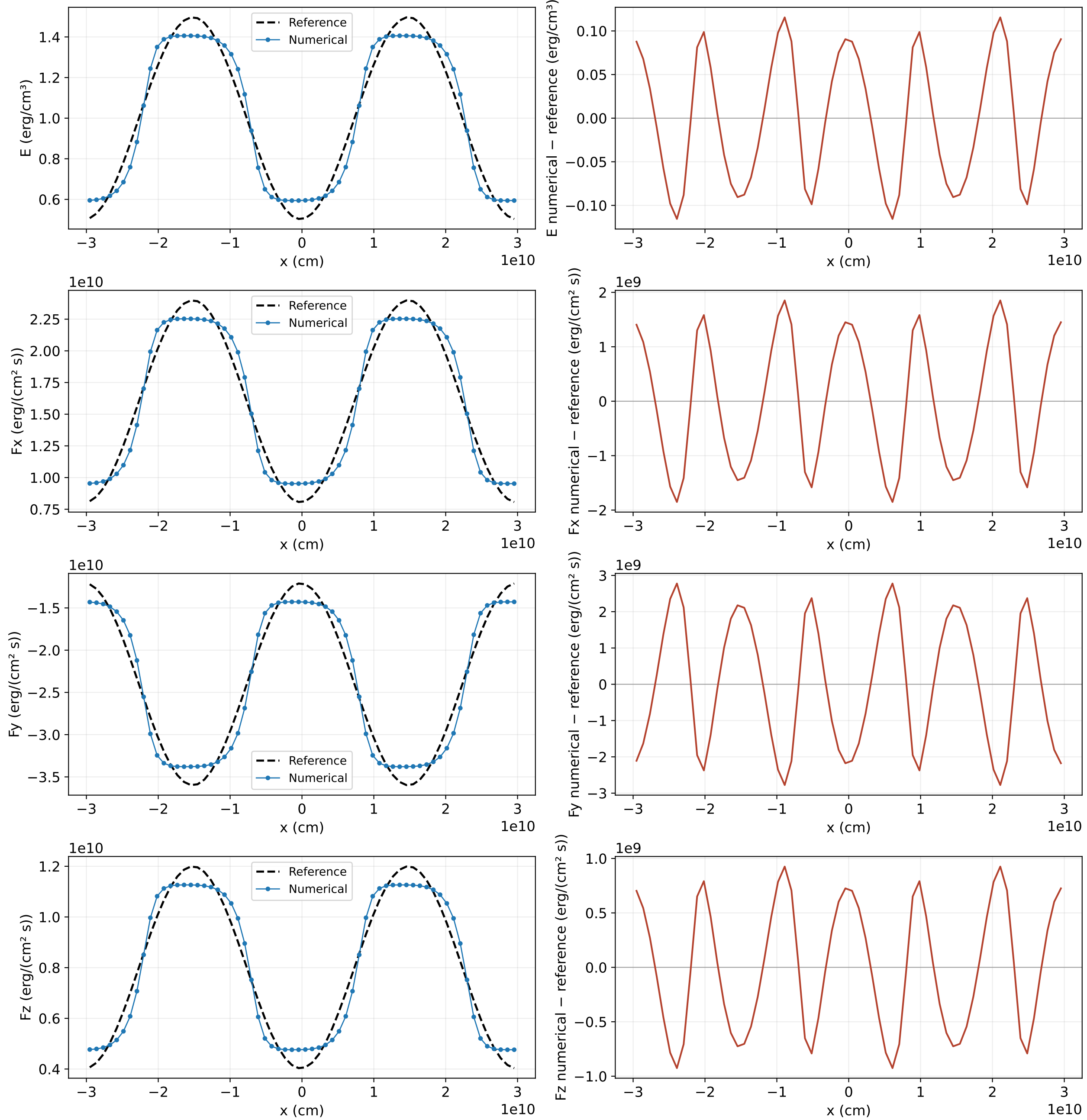
Streaming wave • 64^3 cells • t=4 s • Octo-TIGER application Cell row at y=z=\Delta x/2=4.687500\text{e}+08 cm; matched cell-average reference
