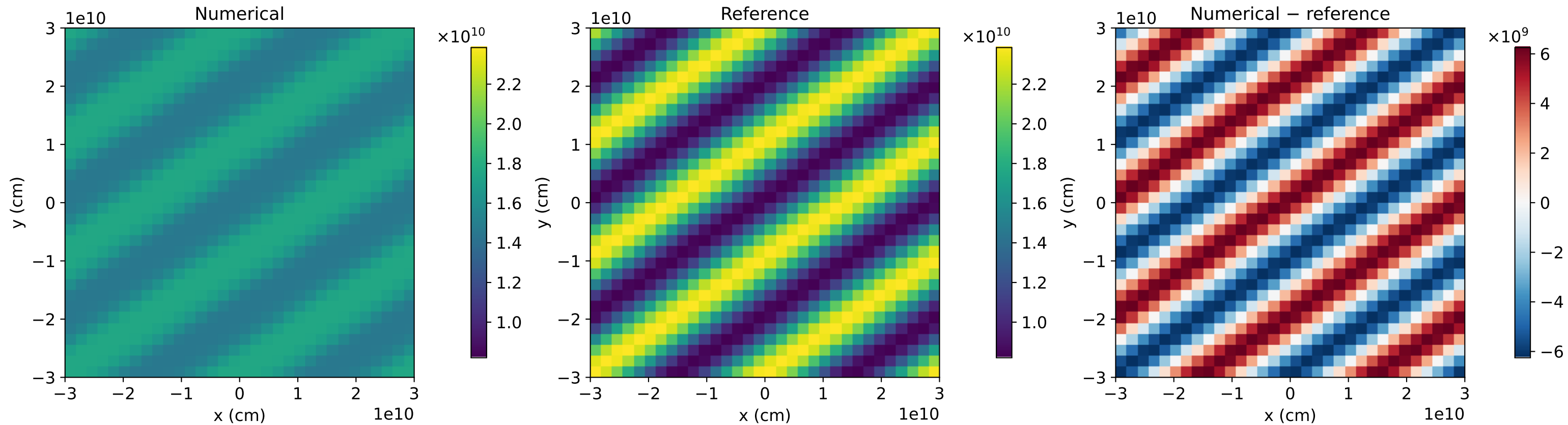
Streaming wave • 32^3 cells • t=4 s • Octo-TIGER application Fx (erg/(cm 2 s)), cell layer at z=\Delta x/2=9.375000\text{e}+08 cm
