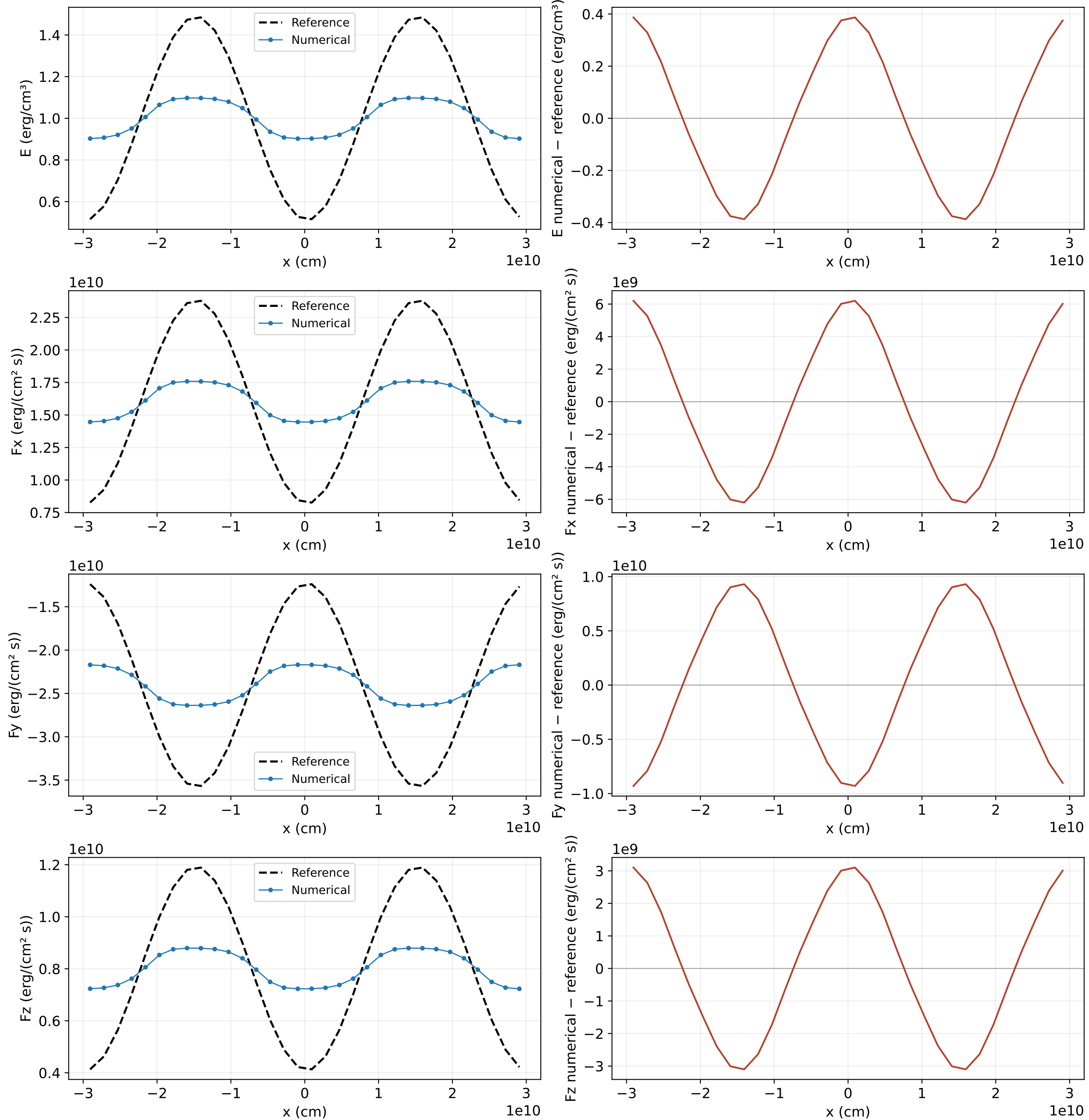
Streaming wave • 32^3 cells • t=4 s • Octo-TIGER application Cell row at y=z=\Delta x/2=9.375000\text{e}+08 cm; matched cell-average reference
