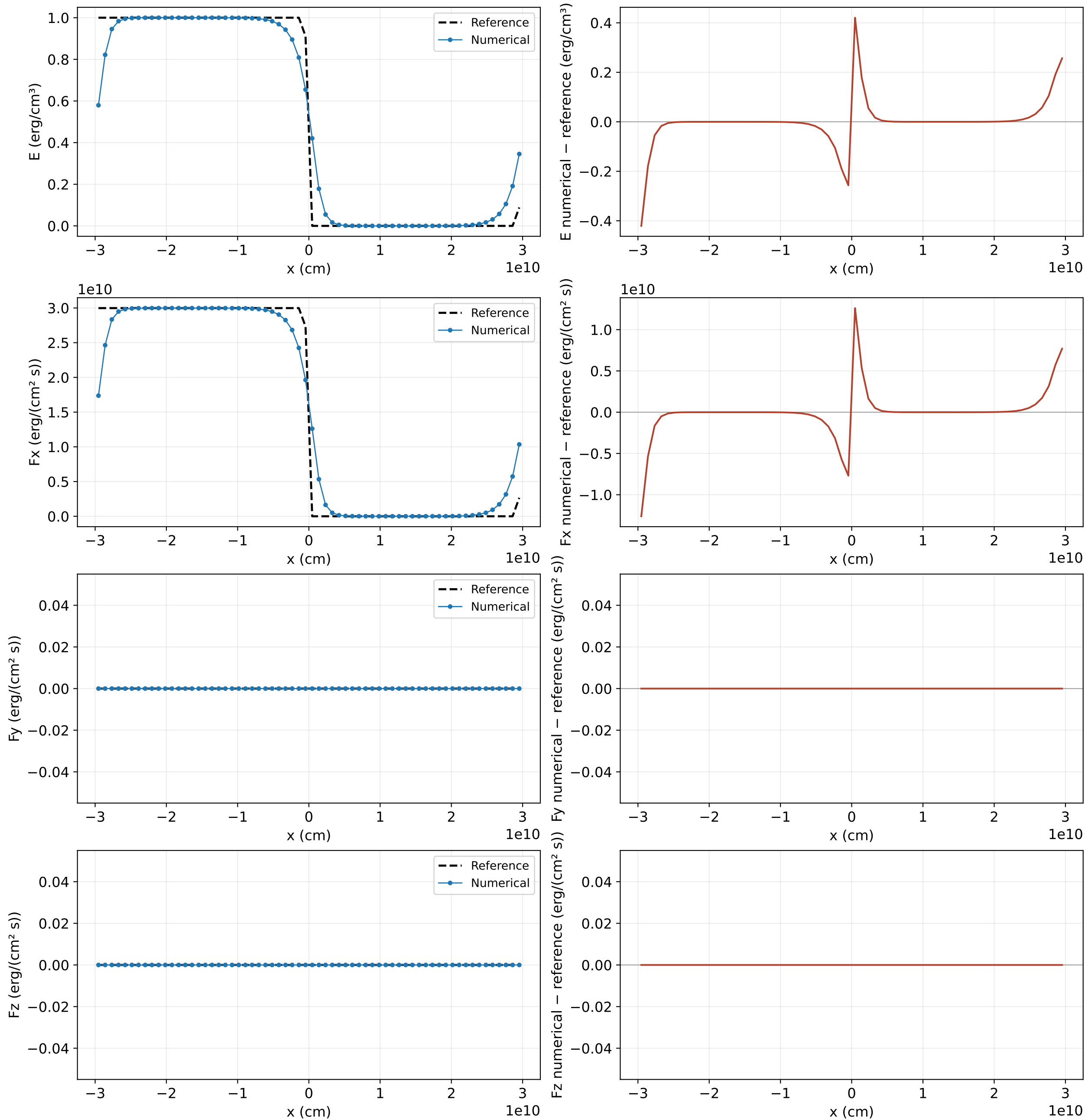
Streaming front • 64^3 cells • t=4 s • Octo-TIGER application Cell row at y=z=\Delta x/2=4.687500\text{e}+08 cm; matched cell-average reference
