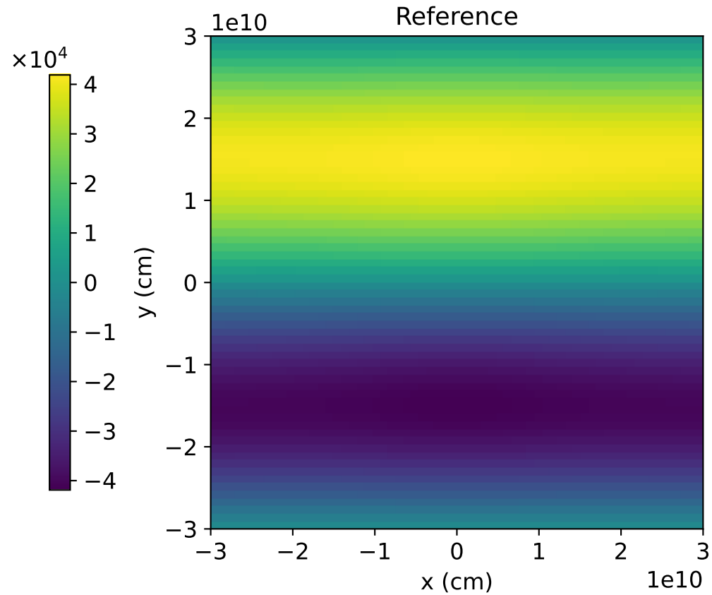
Gaussian pulse • 64^3 cells • t=4 s • Octo-TIGER application F_y (erg/(cm 2 s)), cell layer at z=\Delta x/2=4.687500\text{e}+08 cm
