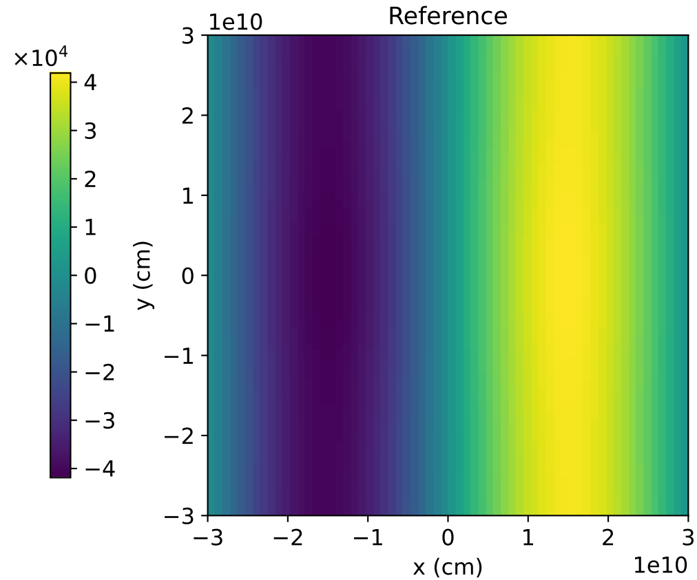
Gaussian pulse • 64^3 cells • t=4 s • Octo-TIGER application Fx (erg/(cm 2 s)), cell layer at z=\Delta x/2=4.687500\text{e}+08 cm
