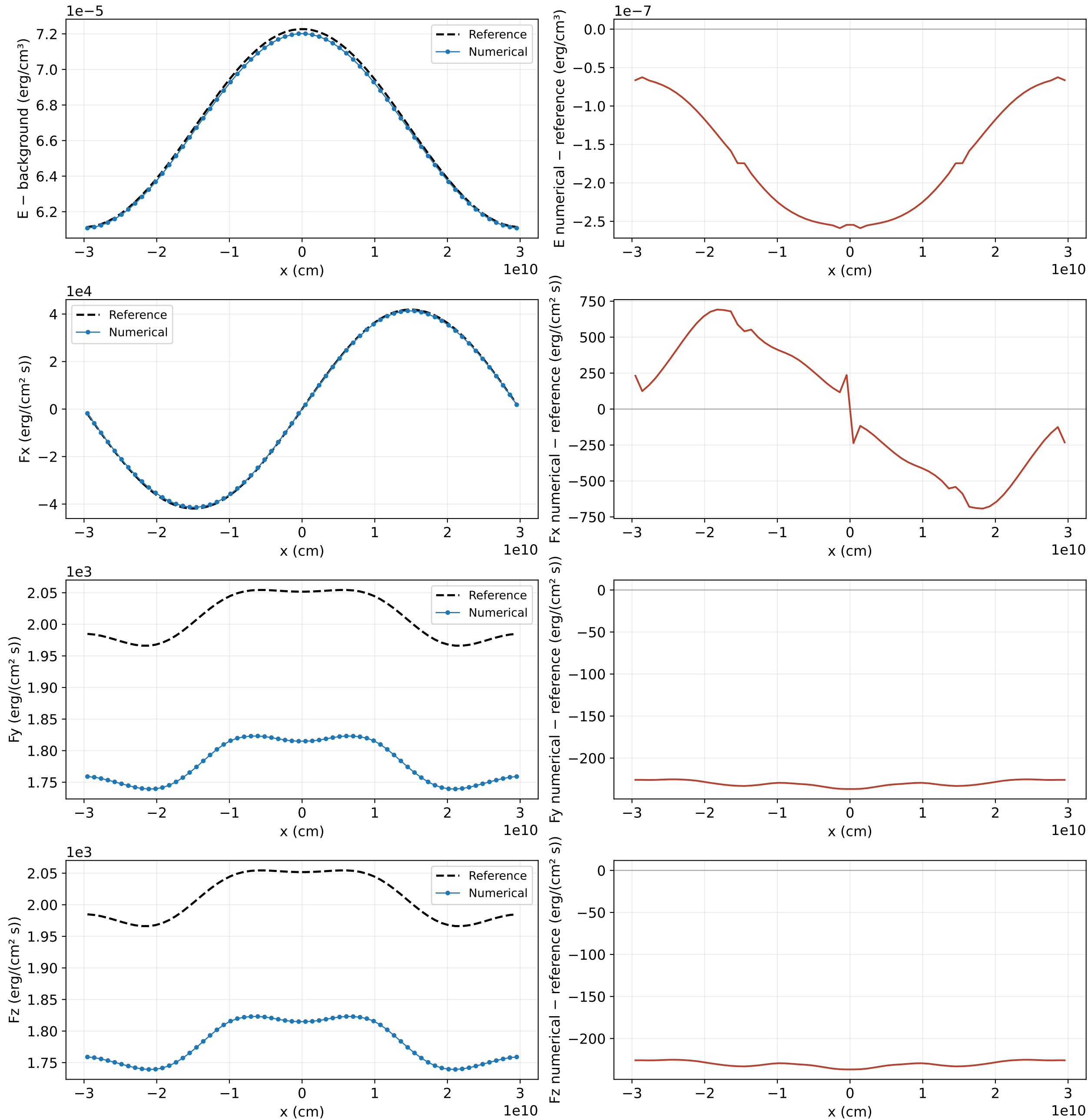
Gaussian pulse • 64^3 cells • t=4 s • Octo-TIGER application Cell row at y=z=\Delta x/2=4.687500\text{e}+08 cm; matched cell-average reference
