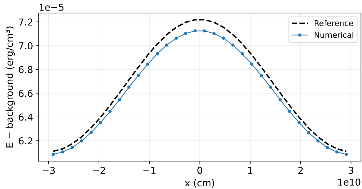
Gaussian pulse • 32^3 cells • t=4 s • Octo-TIGER application Cell row at y=z=\Delta x/2=9.375000\text{e}+08 cm; matched cell-average reference
