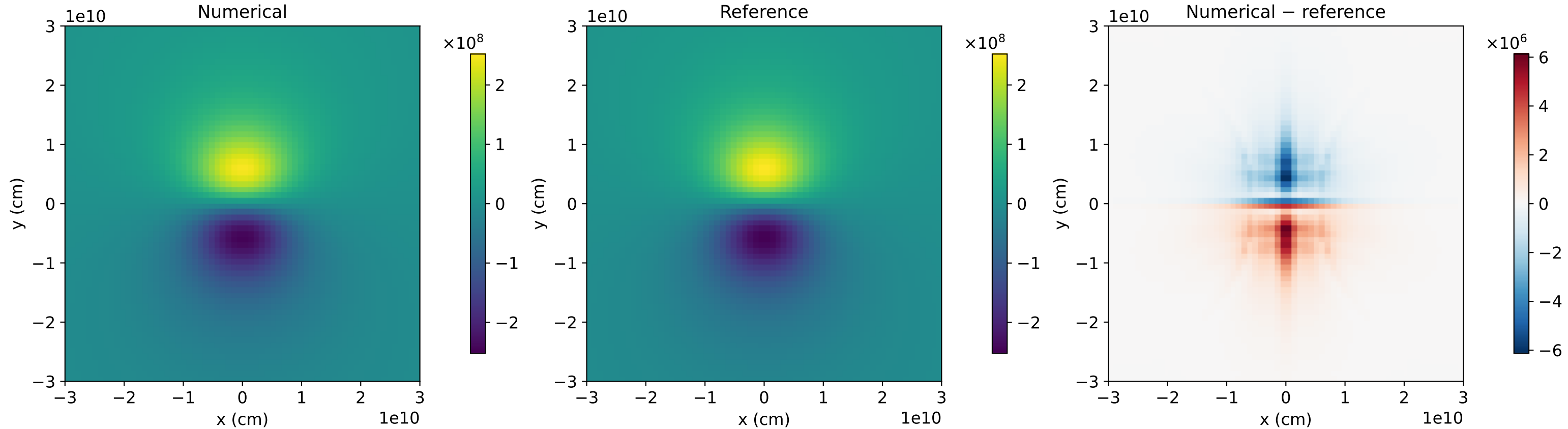
Equilibrium sphere • 64^3 cells • t=4 s • Octo-TIGER application F_y (erg/(cm 2 s)), cell layer at z=\Delta x/2=4.687500\text{e}+08 cm
