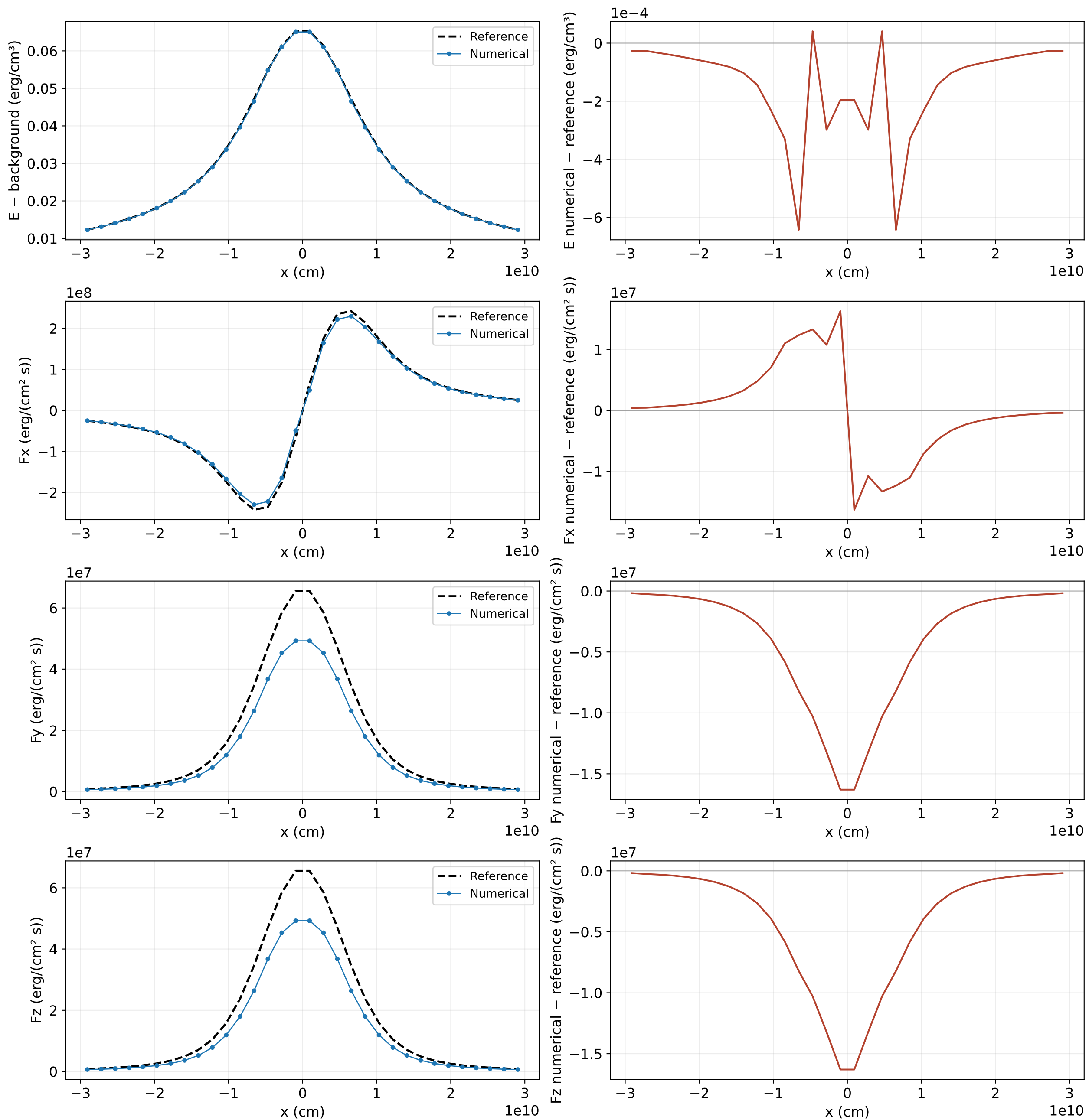
Equilibrium sphere • 32^3 cells • t=4 s • Octo-TIGER application Cell row at y=z=\Delta x/2=9.375000\text{e}+08 cm; matched cell-average reference
